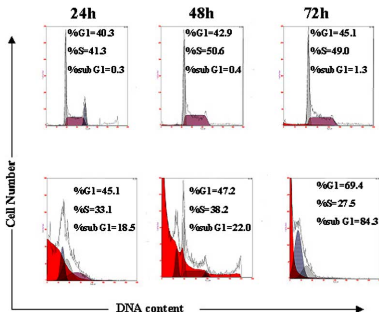
Figure 1. DNA flow cytometric analysis. HL-60 cells were irradiated with compound 12b at concentration of 5 \mu\text{M} and a UVA dose of 2.5 \text{J cm}^{-2} . The cells were harvested for designated times as shown in the figure and described in Ref. 11. The data shown here are from a representative experiment repeated two times with similar results. Upper panels: irradiated controls; lower panels 12b treated cells.
